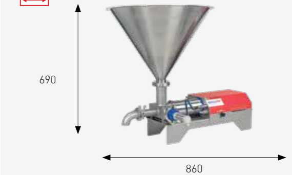
- Dimensions (L x H): 860 x 690 mm
